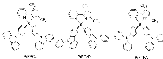
Scheme 1. Structural drawings of the boron complexes, PrFPCz , PrFCzP , and PrFTPA .
